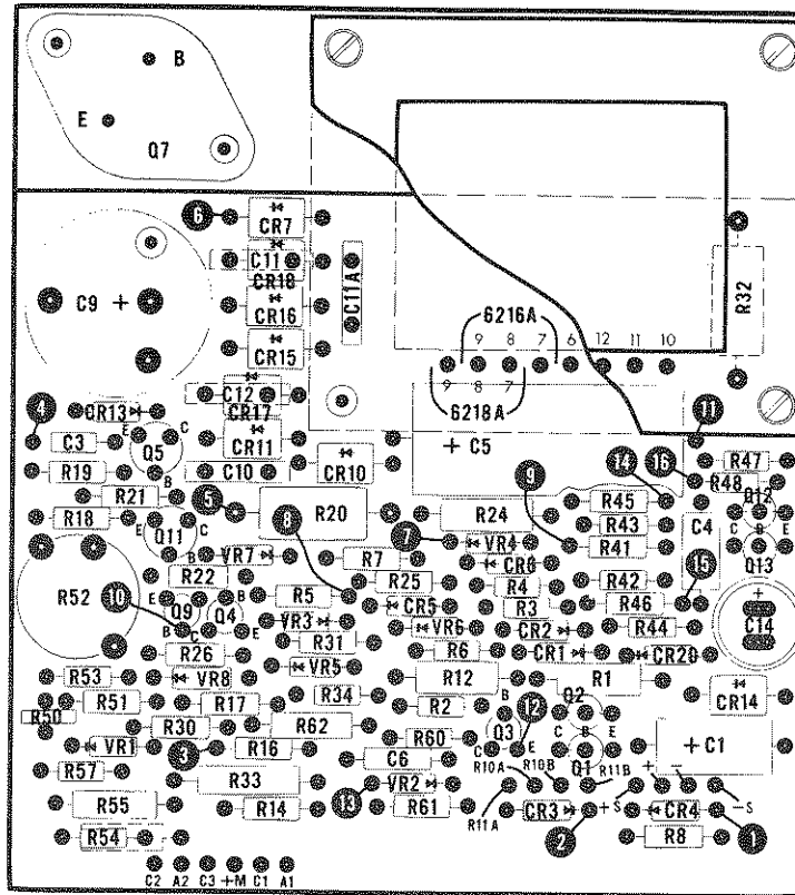
Figure A-3. Model 6216A, Component Location Diagram
